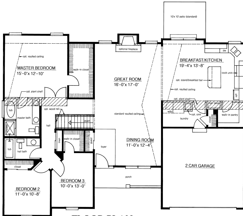
FLOOR PLAN
