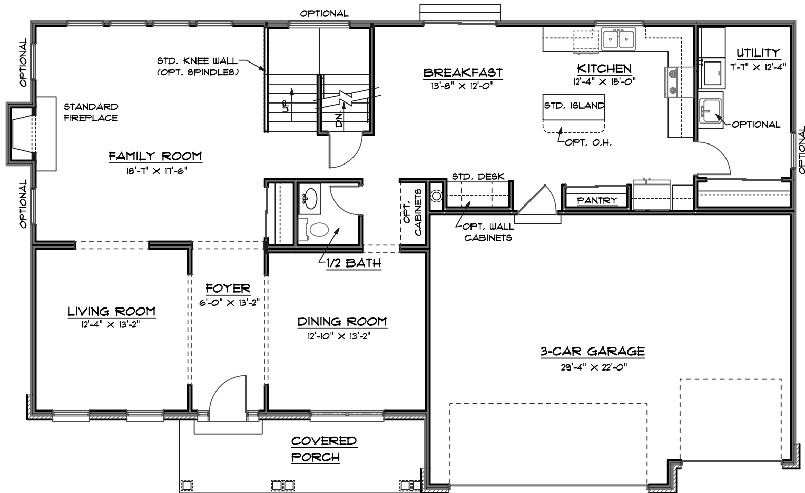
"WILLOW" FIRST FLOOR PLAN
