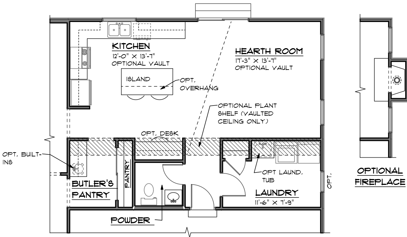
OPTIONAL HEARTHROOM PLAN
