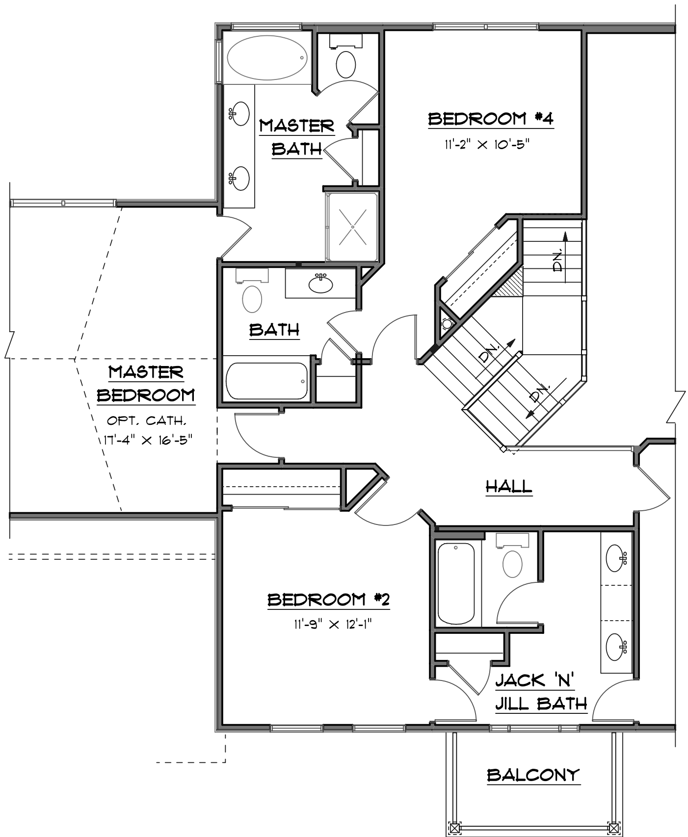
"POPLAR 2ND FLOOR PLAN OPTION A"
