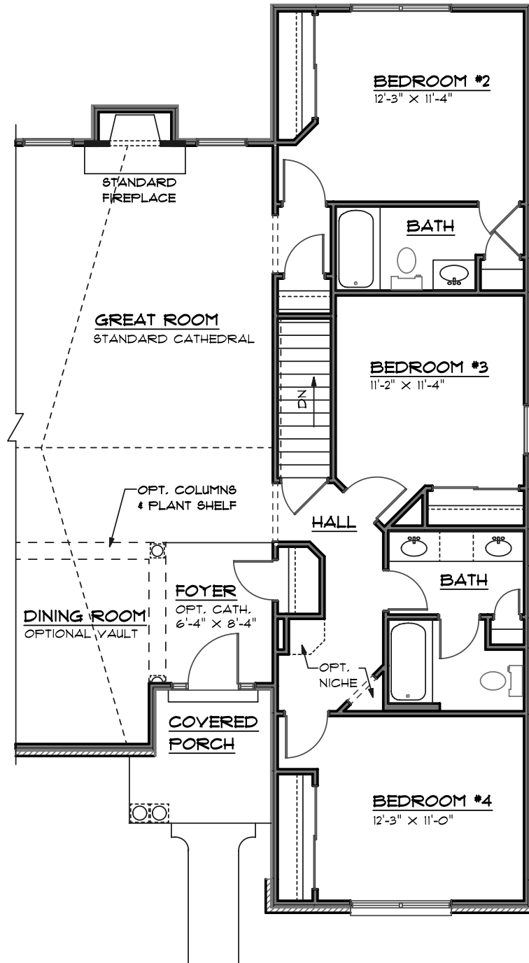
CYPRESS FOUR BEDROOM FLOOR PLAN "C"
