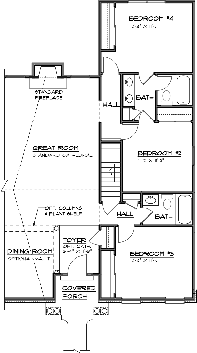
CYPRESS FOUR BEDROOM FLOOR PLAN "B"
