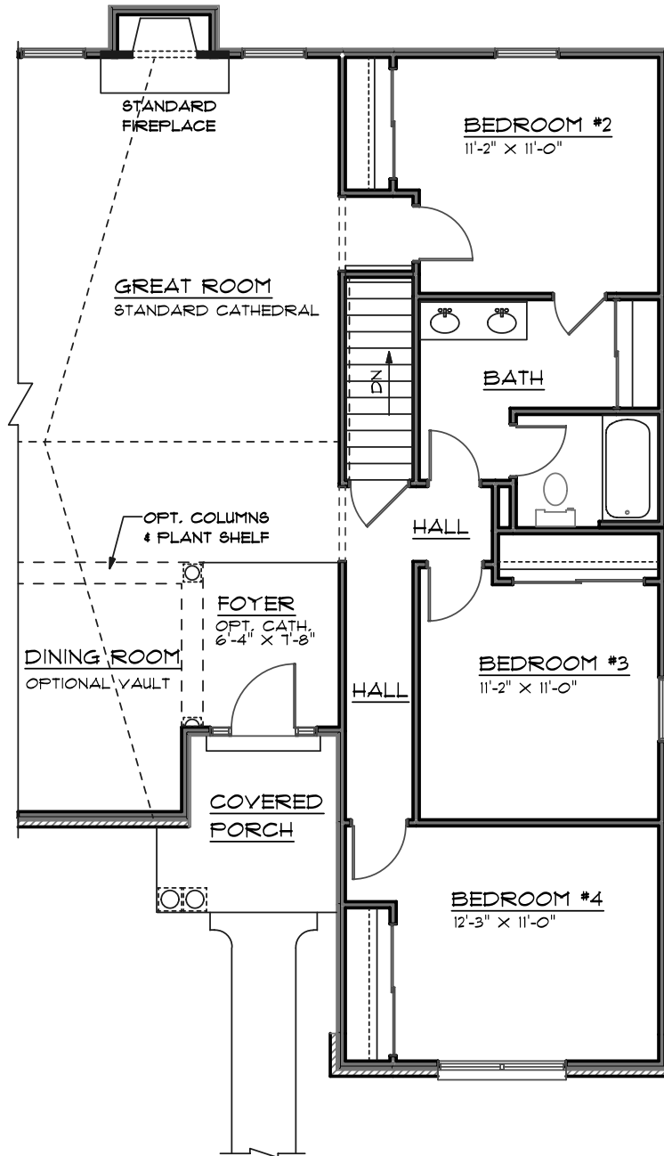
CYPRESS FOUR BEDROOM FLOOR PLAN "A"
