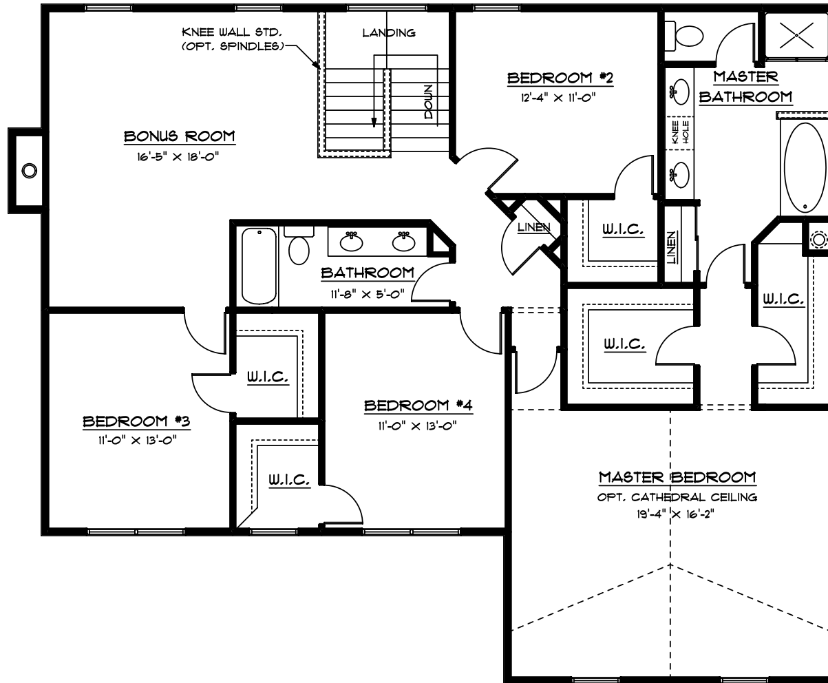
"BIRCH" 2ND FLOOR PLAN
