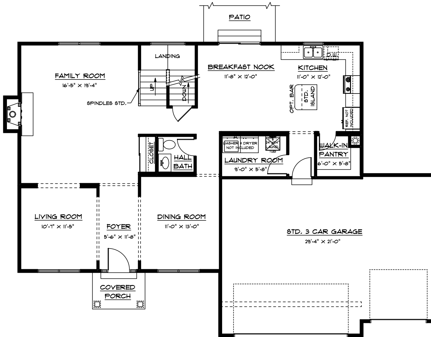
"BIRCH" 1ST FLOOR PLAN
